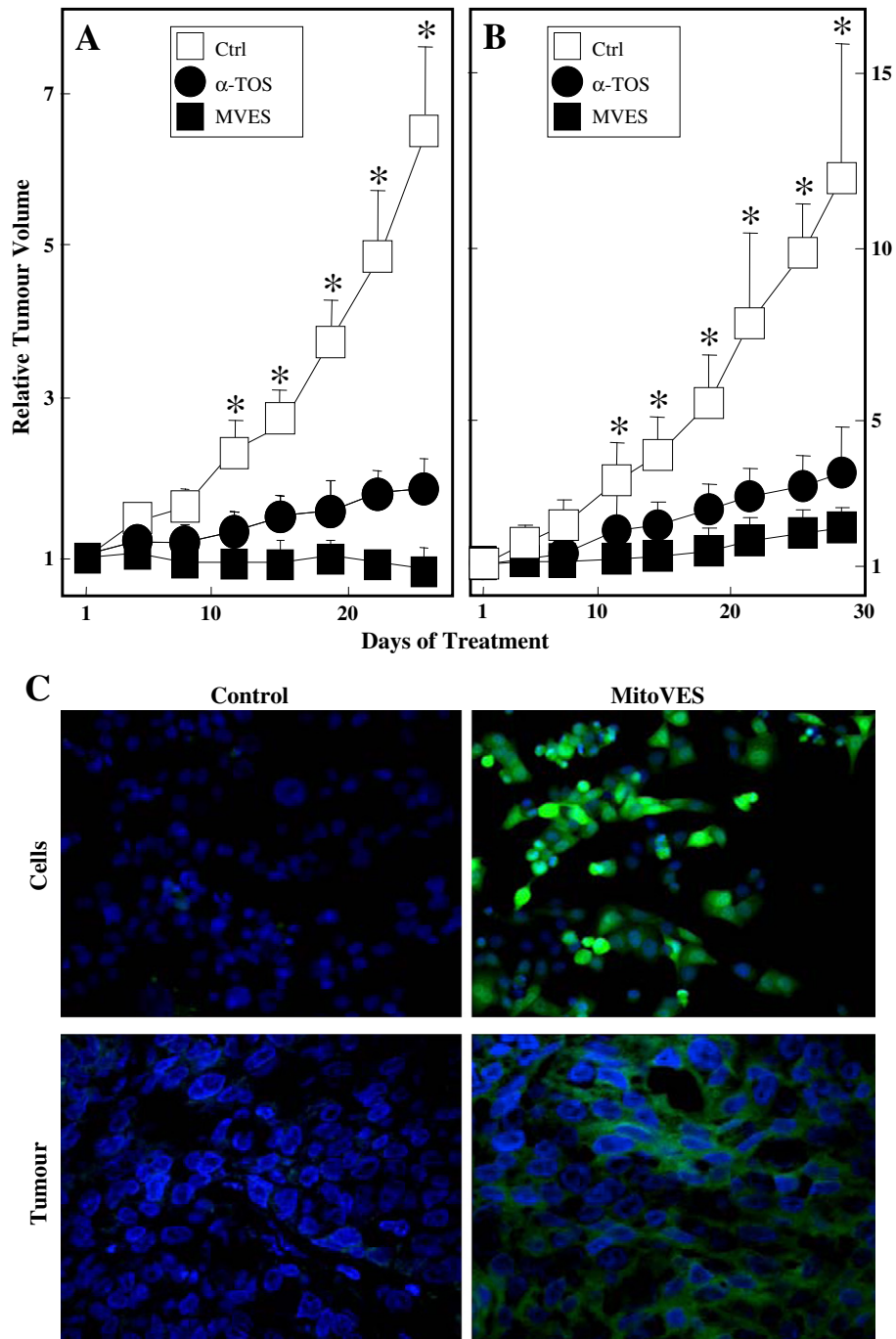
Fig. 5. MitoVES efficiently suppresses tumours and induces pseudohypoxia in cancer cells and in tumours. FVB/N c-neu transgenic mice with spontaneous breast carcinomas (A) and nude mice with xenografts derived from colorectal HCT116 cells (B) were treated with \alpha -TOS and with MitoVES at 10-fold lower doses than that of the former. Ultrasound imaging documents a superior activity of MitoVES over its untargeted counterpart. C. HCT116 colon cancer cells were stably transfected with the ODD-GFP gene-containing plasmid. The cells were exposed to 5 \mu M MitoVES for 12 h and green colour, indicative of the accumulation of the chimeric ODD-GFP protein observed using confocal microscopy (upper images). Sections from HCT116 ODD-GFP -derived tumours treated with MitoVES were inspected by confocal microscopy, revealing green fluorescence. The in vitro and in vivo experiments document that the mechanism by which MitoVES induces apoptosis is similar in both settings. Adapted from [80] and [116].
