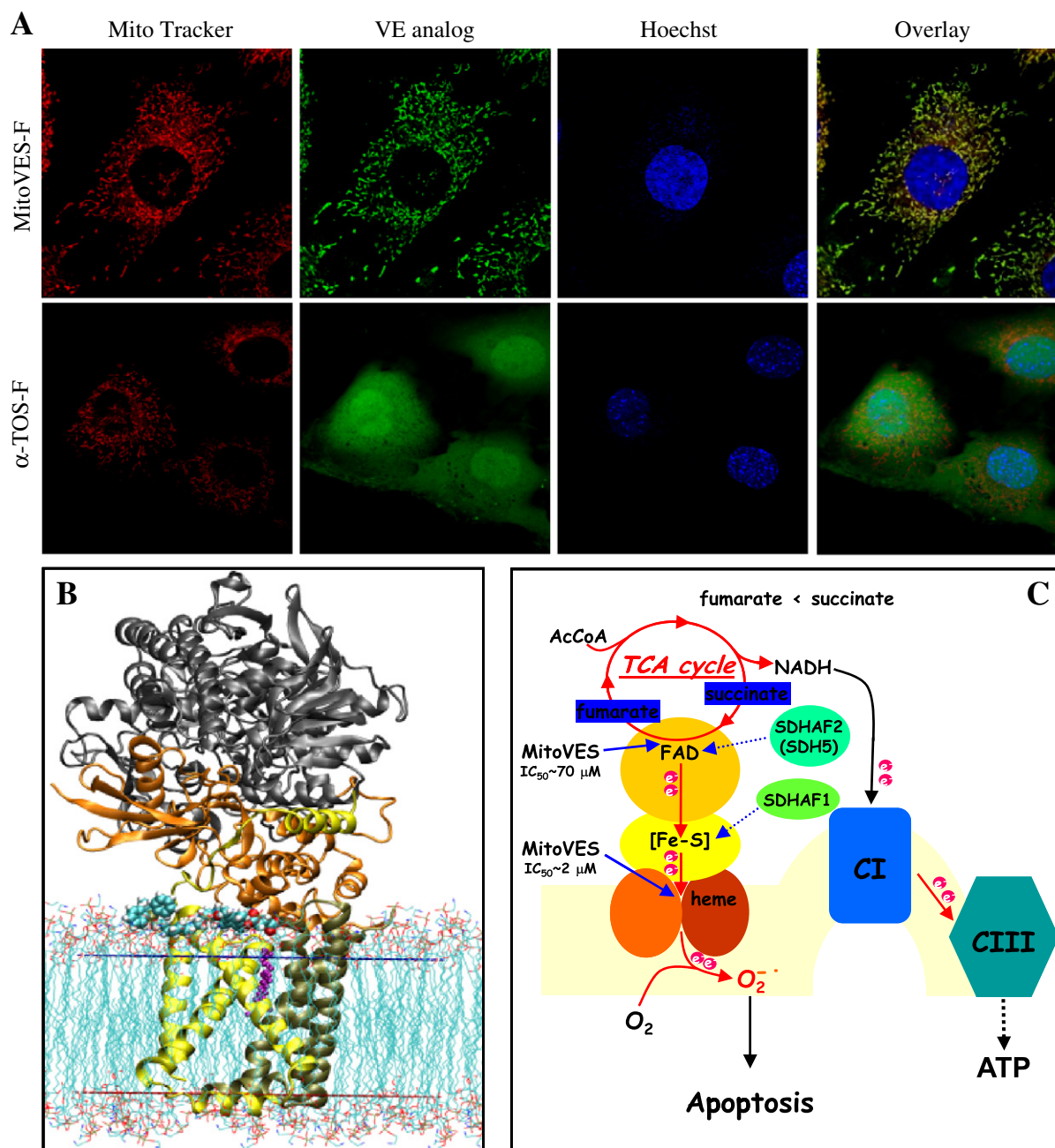
Fig. 4. Mitochondrial localisation of MitoVES, its interaction with CII and the molecular mechanism of its effect on CII. A. Mouse breast cancer NeuTL cells were incubated with MitoTracker Red and fluorescently labelled MitoVES or \alpha -TOS and inspected by confocal microscopy. Hoechst 33342 was used to visualise the nuclei. B. Molecular modelling indicated the position of MitoVES at the interface of the MIM and matrix components of CII. C. MitoVES inhibits both SDH and SQR activity of CII, the former with IC_{50} \sim 70 \mu M , the latter with IC_{50} \sim 2 \mu M . Due to this scenario, the conversion of succinate to fumarate occurs in the presence of MitoVES, albeit at a lower rate, generating electrons that are forced to transverse to the membrane components of CII. In the situation when UbQ is displaced from the Q_p site in CII, electrons lack their natural acceptor and recombine with molecular oxygen to give rise to superoxide. This then triggers a series of reactions that result in the induction of the apoptotic cascade, resulting in the demise of the cell. Adapted from [19,80,116].
