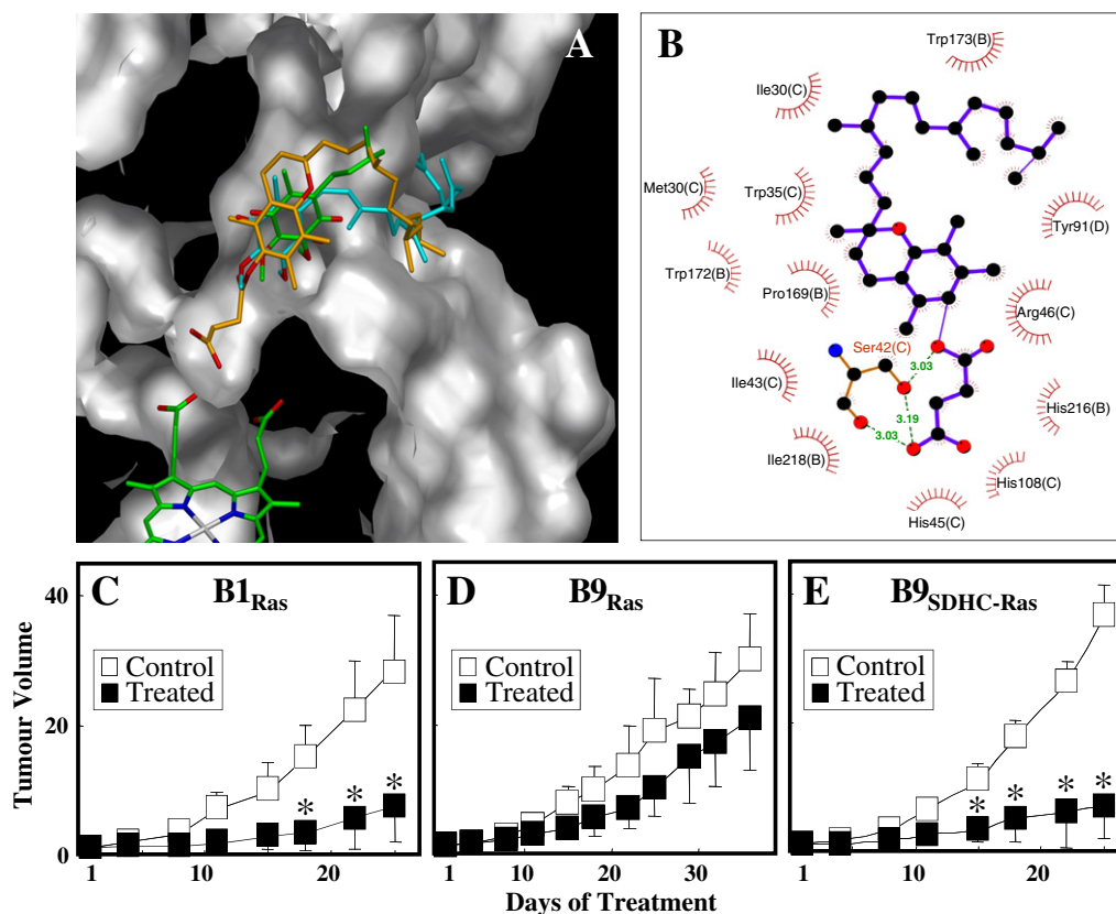
Fig. 3. Model of the interaction of \alpha -TOS with CII and its effect on CII-functional and dysfunctional tumours. Molecular modelling indicates the position of \alpha -TOS in relation to UbQ and heme between the SDHC and SDHD subunits of CII (A), and its interaction with the Ser68 (shown here as Ser42 as used in the study by Sun et al. [34], which binds UbQ in the Q_p site. Strong hydrogen bonds of the oxo groups of the succinyl moiety of \alpha -TOS with the SDHC's Ser68 are indicated (B). Parental B1, SDHC-deficient B9 and SDHC-reconstituted B9 SDHC cells were transformed with H-Ras and grafted into nude mice to form tumours. The carcinomas were treated with \alpha -TOS, indicating a good response of the CII-functional and very little response of the CII-compromised tumours (C–E). Adapted from [26] and [116].
